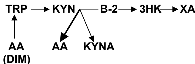
Figure 3. Hypothetical changes of Tryptophan-Kynurenine metabolism in T1D.
