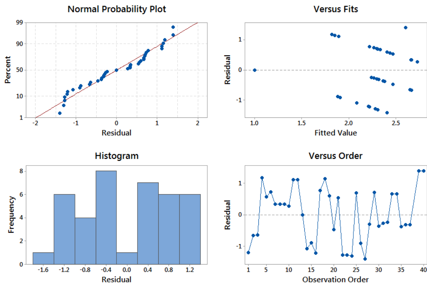
Figure 2. Representative graphs showing the results of the Durbin-Watson residual analysis.
